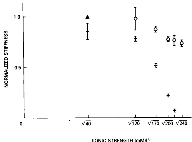
FIGURE 3 Summary of the ionic strength dependence of fiber stiffness in the presence of 4 mM MgPP_i obtained from four fibers at 6°C. O, in the presence of PP_i and \text{Ca}^{2+} ; +, in the presence of MgPP_i but absence of \text{Ca}^{2+} . Data normalized to the rigor stiffness at \mu = 40 mM ( \Delta ). Sarcomere length = 2.3 \mu\text{m} . Temperature = 6^\circ\text{C} . Error bars show \pm\text{SEM} .
