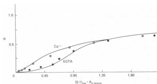
FIGURE 1 Binding of S1-PP i to regulated actin at 6°C, \mu = 35 mM, in the presence (○) and absence (●) of Ca 2+ . ○ is moles of S1 bound per mole of F-actin monomer. Smooth curves are calculated from the model of Hill et al. (1980) assuming K_{(\text{strong})} = 4.5 \times 10^4 \text{ M}^{-1} , K_{(\text{weak})} = 5 \times 10^3 \text{ M}^{-1} , Y = 5 , and L' = 30 for +Ca 2+ and 2 for -Ca 2+ . Similar values were obtained from two other experiments.
