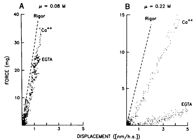
FIGURE 2 Original records showing force versus change in sarcomere length during stretches of a single skinned rabbit psoas fiber. The slope of the relationship gives the fiber stiffness. The speed of stretch was \sim 5 \times 10^3 nm/half-sarcomere/s. The bathing solutions contained 4 mM MgPP_i , with or without \text{Ca}^{2+} ; T = 6^\circ\text{C} . Dashed line shows the rigor stiffness. In A, \mu = 80 mM; in B, \mu = 220 mM.
